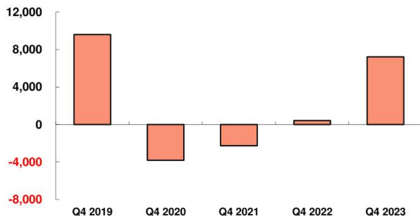
Operating Income
